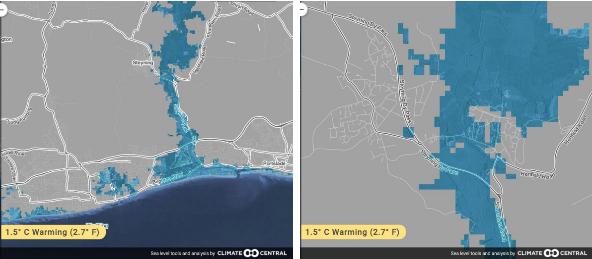
Figure 2: Predicted coastal inundation by 2200 for the Adur Valley (left) and Steyning (right) assuming a 1.5°C rise in global temperatures 7
