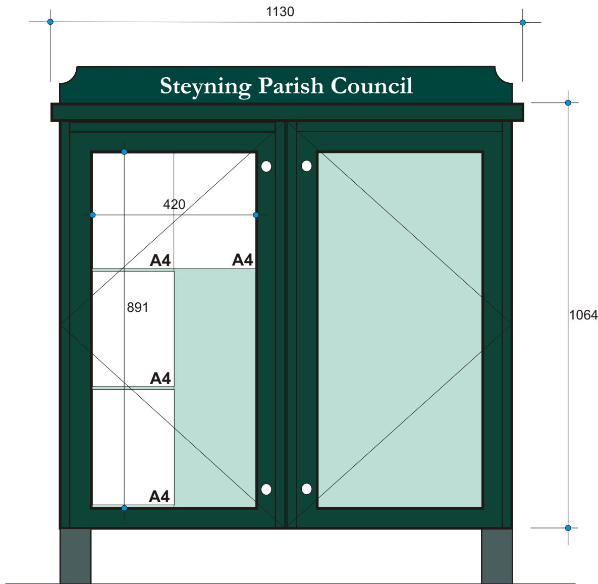
FRONT ELEVATION
